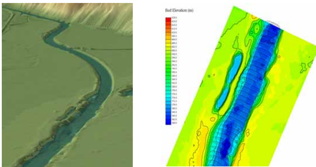
Fig 1: Shaded DTM of river Drau and the result of an applied hydraulic model
