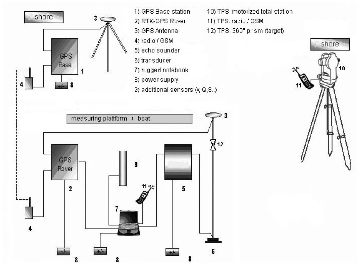
Fig.4: Configuration of the measuring system
